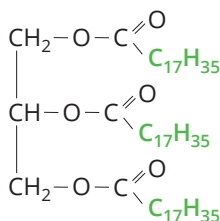
tristearynian glicerolu
