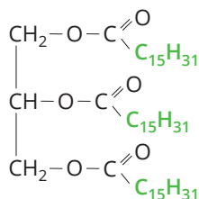
tripalmitynian glicerolu
