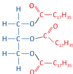
tristearynian glicerolu
