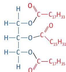
1-oleinian-2-palmitynian-3-stearynian glicerolu
