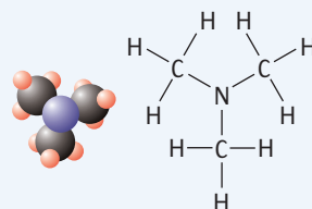
trimetyloamina
