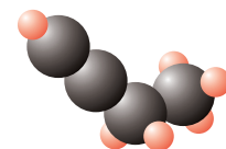
▲ Model but-1-ynu
