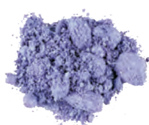
Cr 2 (SO 4 ) 3
