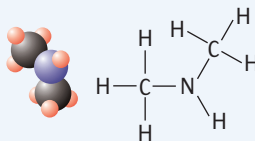
dimetyloamina
